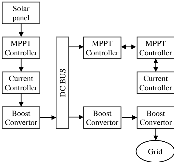
Fig.1. Proposed PV power grid
