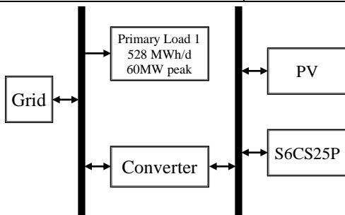
Fig.4. HOMER Solar Grid
