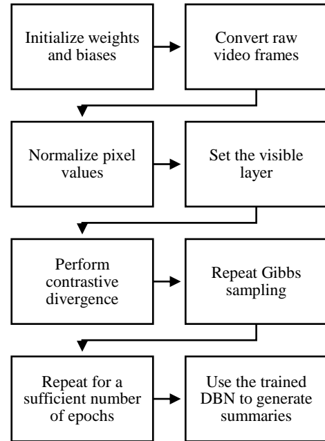
Fig.1. Feature Extraction (Video Summarization using DBN)
