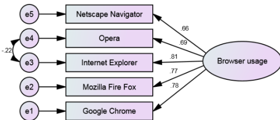
Fig.5. Measurement model for browser usage
