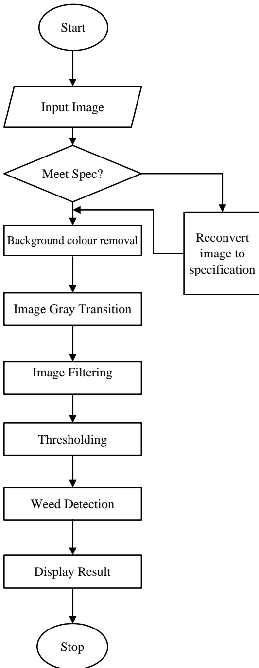
Fig.4. Flowchart for weed detection system
