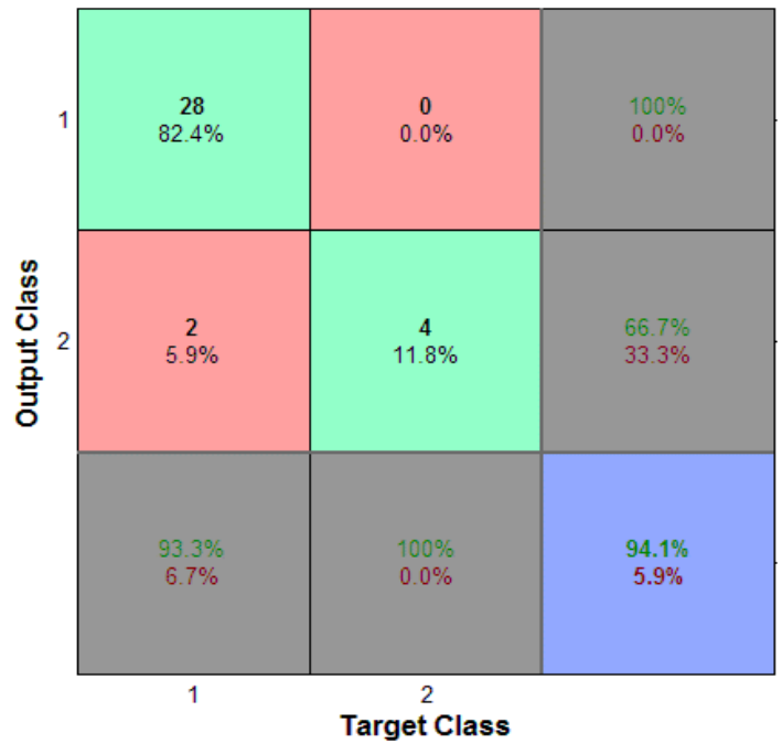
Fig.7. Confusion Matrix
