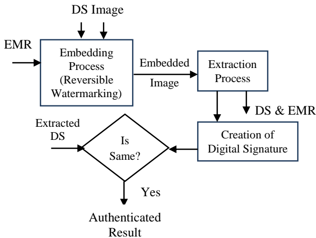
Fig.2. Embedding and Extraction Procedure
