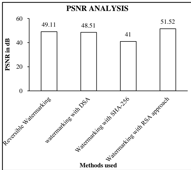
Fig.3. PSNR Analysis
