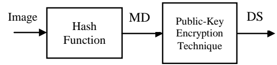
Fig.1. Creation of Digital Signature
