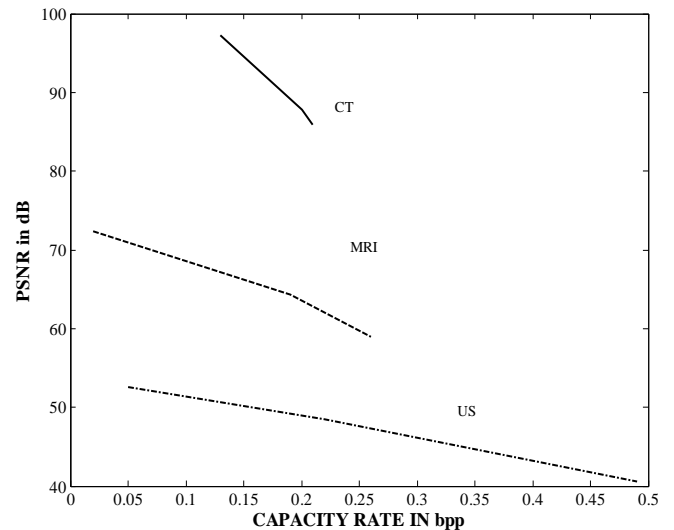
Fig.4. Analysis of PSNR for various Capacity Rate in different Modalities
