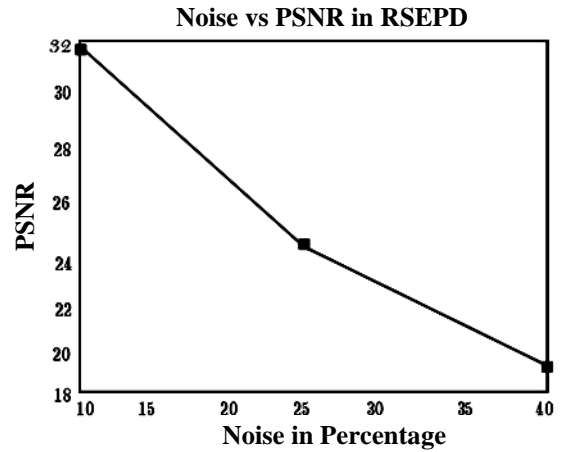
Fig.15. Graphical representation of PSNR values vs various percentage of noise in RSEPD
