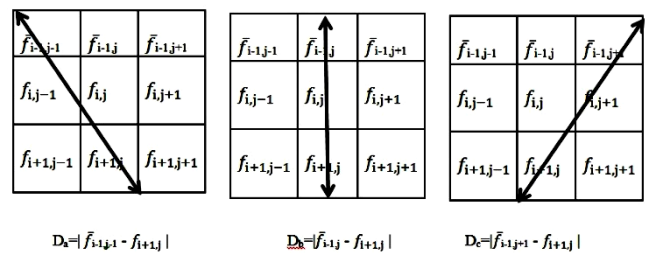
Fig.11. Three edge lines of RSEPD
