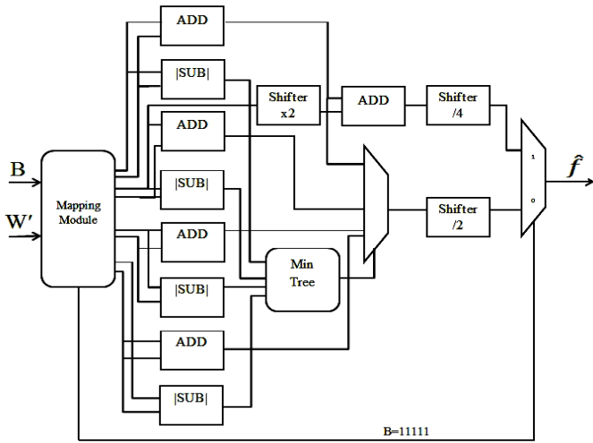
Fig.5. Architecture of edge oriented noise filter
