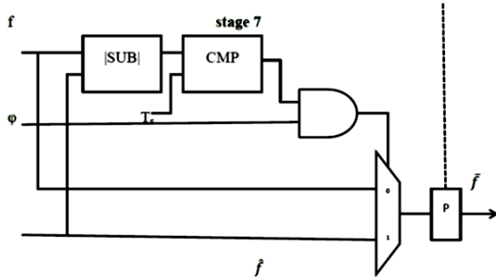
Fig.8. Architecture of impulse arbiter
