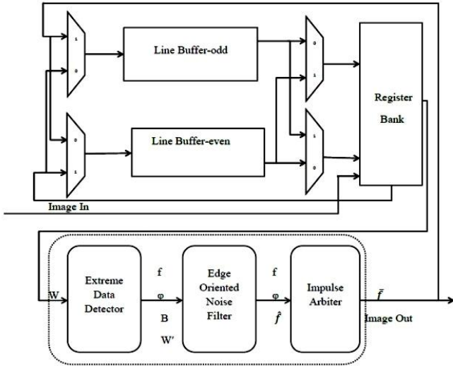
Fig.1. SEPD Architecture
