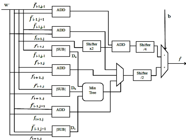
Fig.13. Edge oriented noise filter
