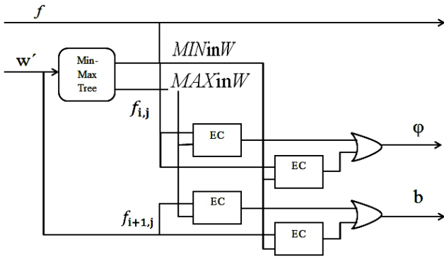
Fig.12. Extreme data detector architecture
