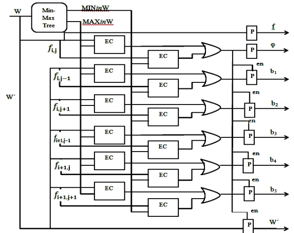
Fig.4. Extreme data detector architecture
