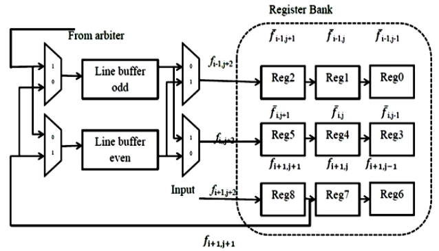
Fig.3. Register bank architecture
