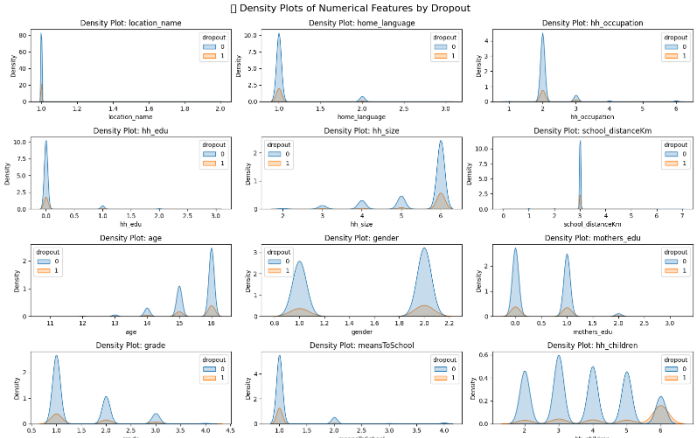
Fig.1. Density plot of Numerical Features by Dropouts
