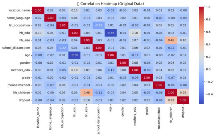
Fig.2. Correlation Heatmap
