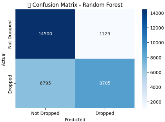
Fig.7 Confusion matrix – Random Forest
