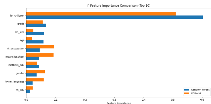
Fig.9. Feature Importance mechanism
