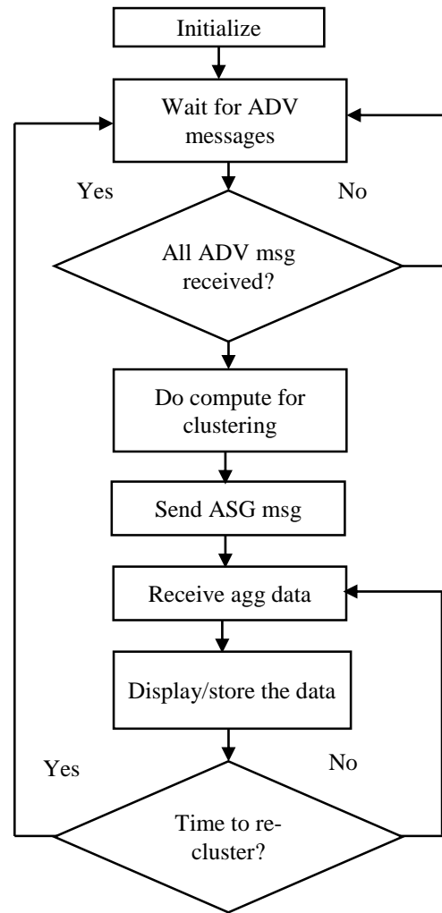
Fig.4. Flow chart of network operation at the BS
